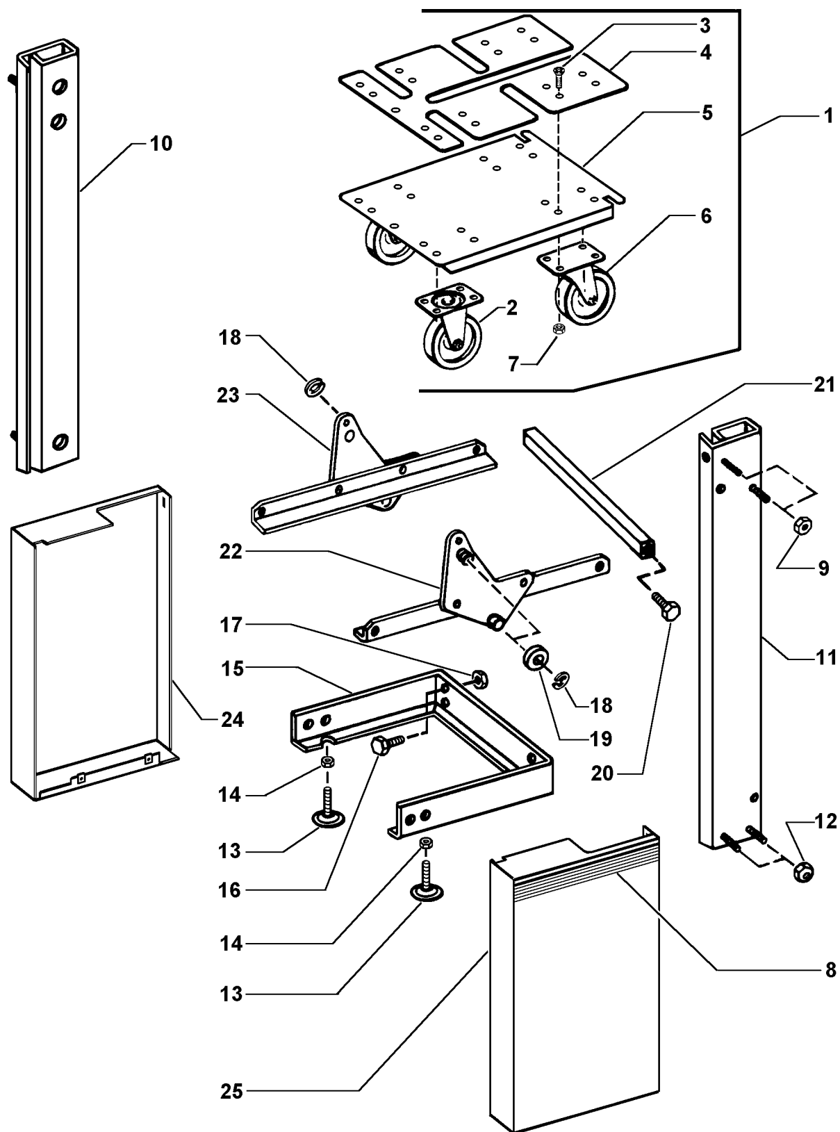
FIGURE 82 Dolly and Frame Assemblies
