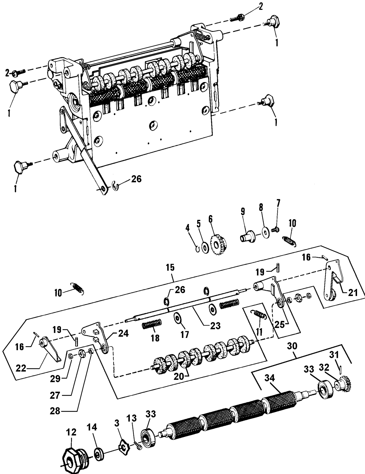
FIGURE 50 Main Tie Bar Assembly - Part I
