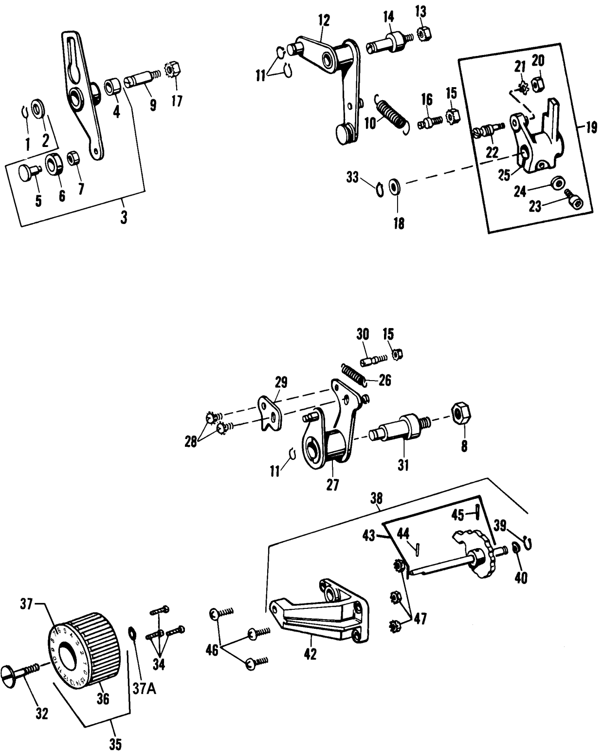
FIGURE 46 Buckle Adjusting and Lever Assemblies
