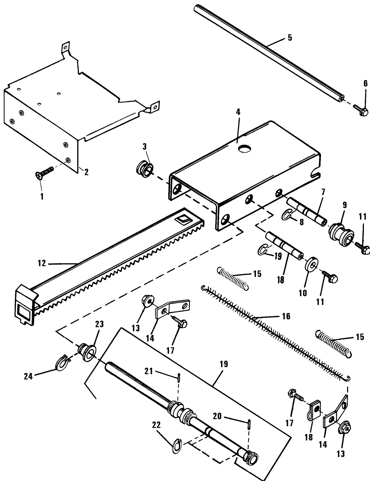
FIGURE 74 Back Jogger Mechanism - Part I
