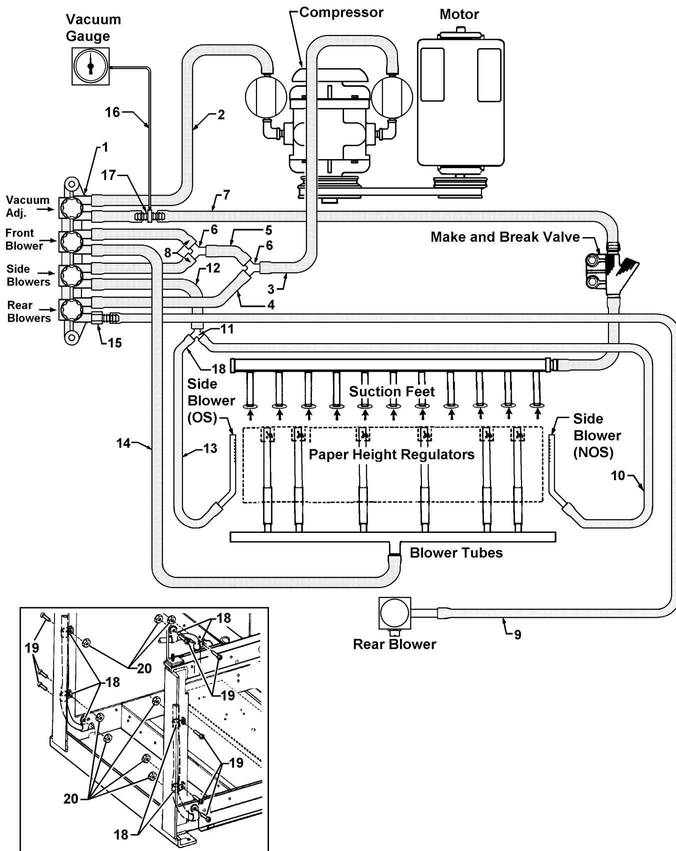
FIGURE 59 Air and Vacuum Assemblies - Part II
