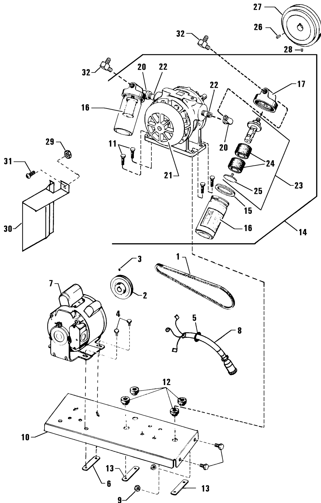
FIGURE 60 Compressor Assembly
