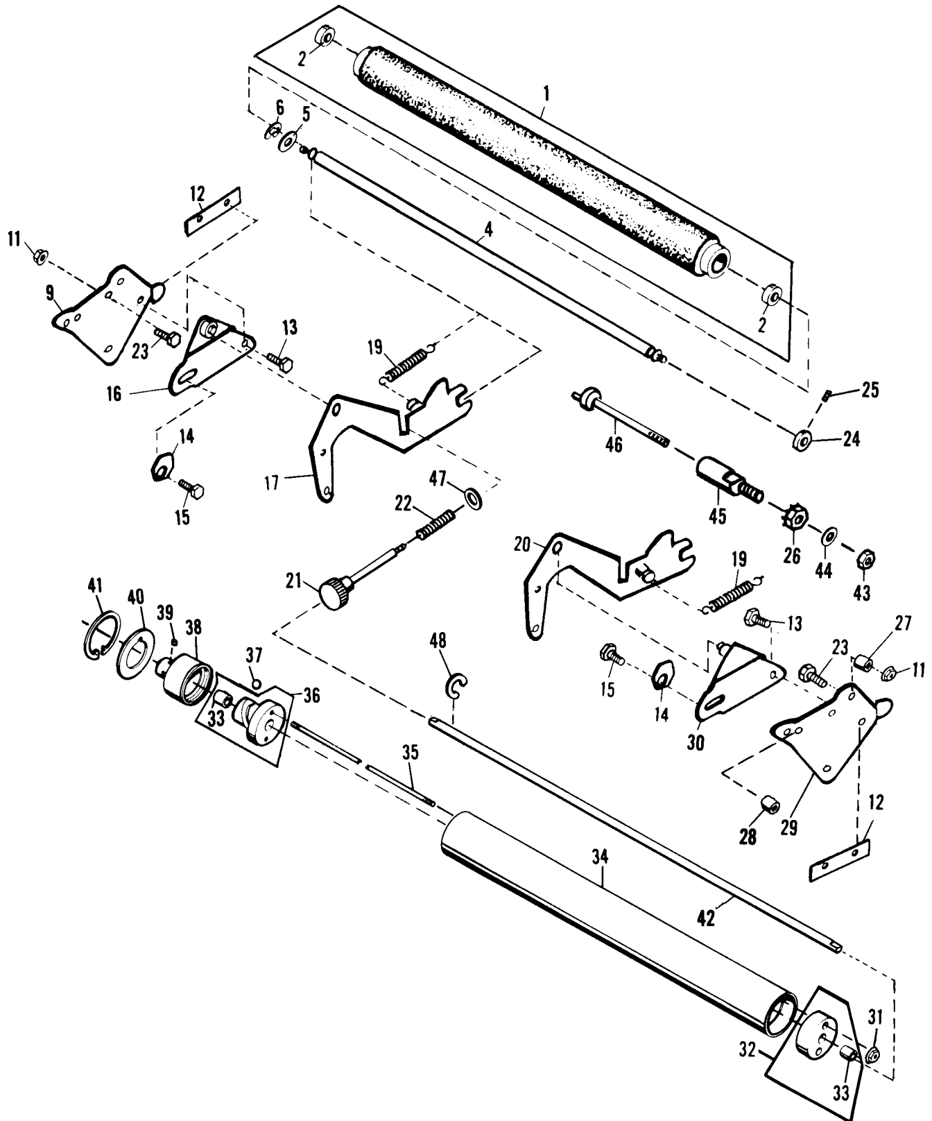
FIGURE24 Form Roller - Third
