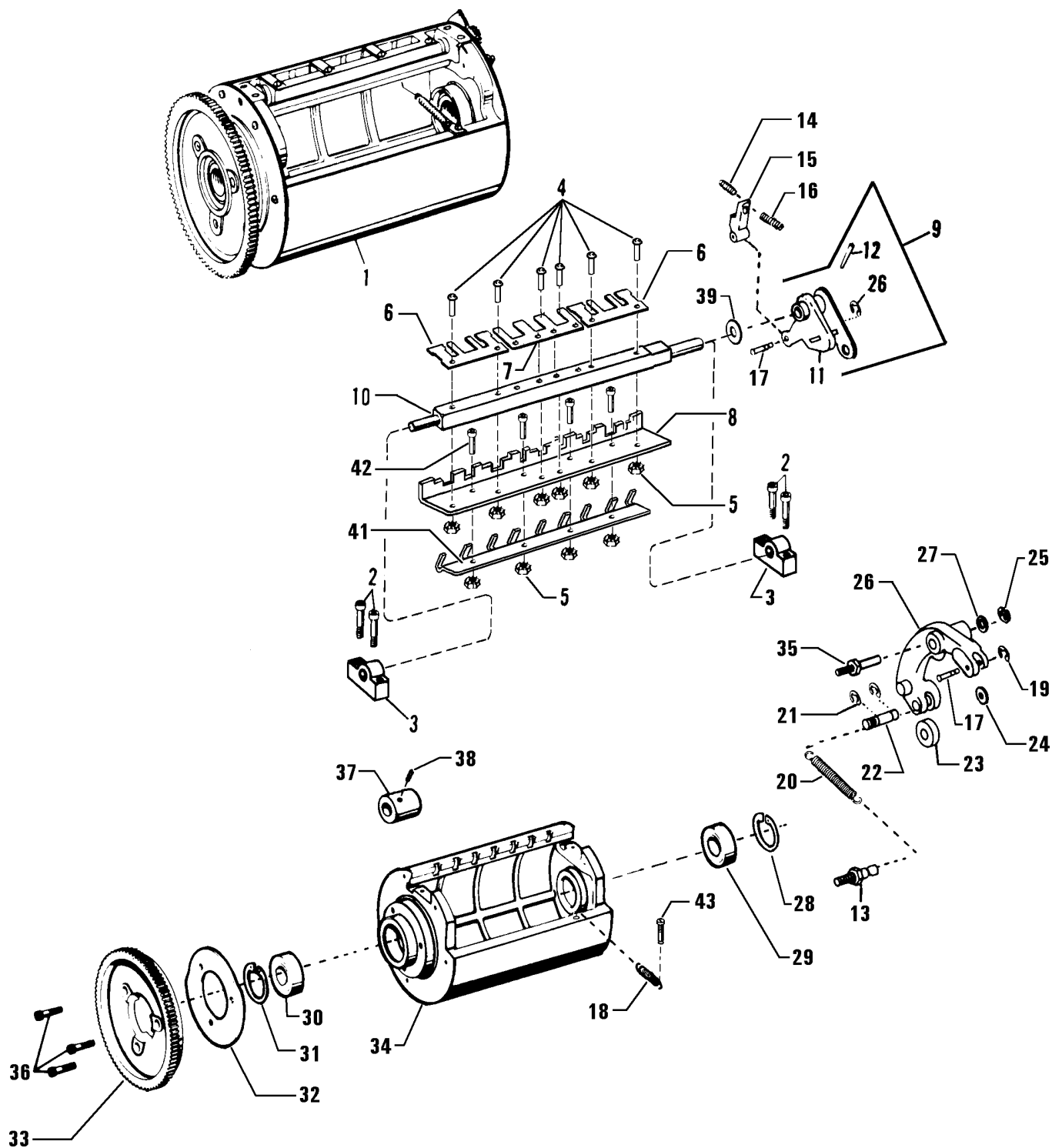
FIGURE 38 Impression Cylinder Assembly
