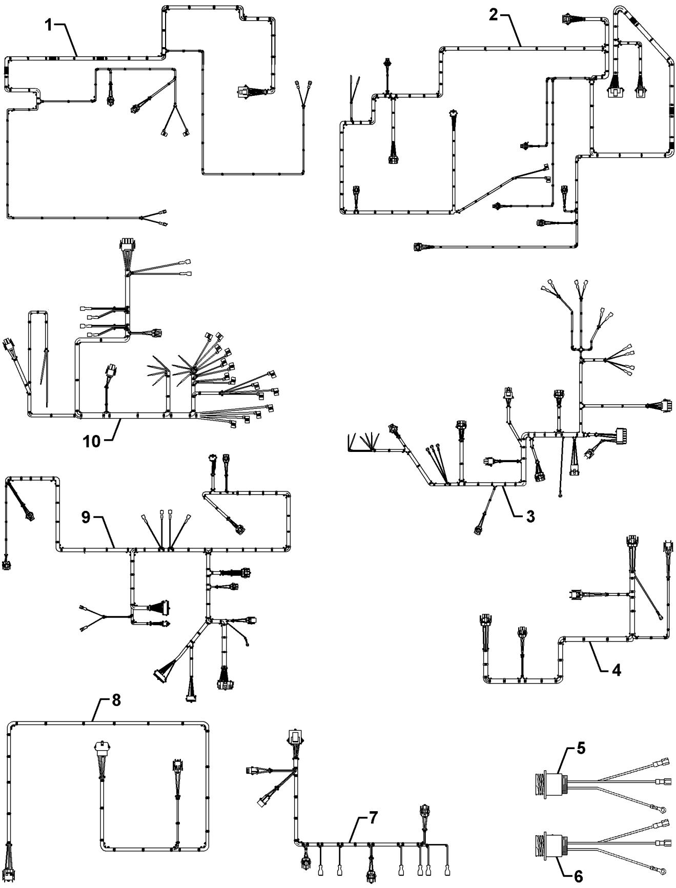
FIGURE 68 Control Box Harnesses
