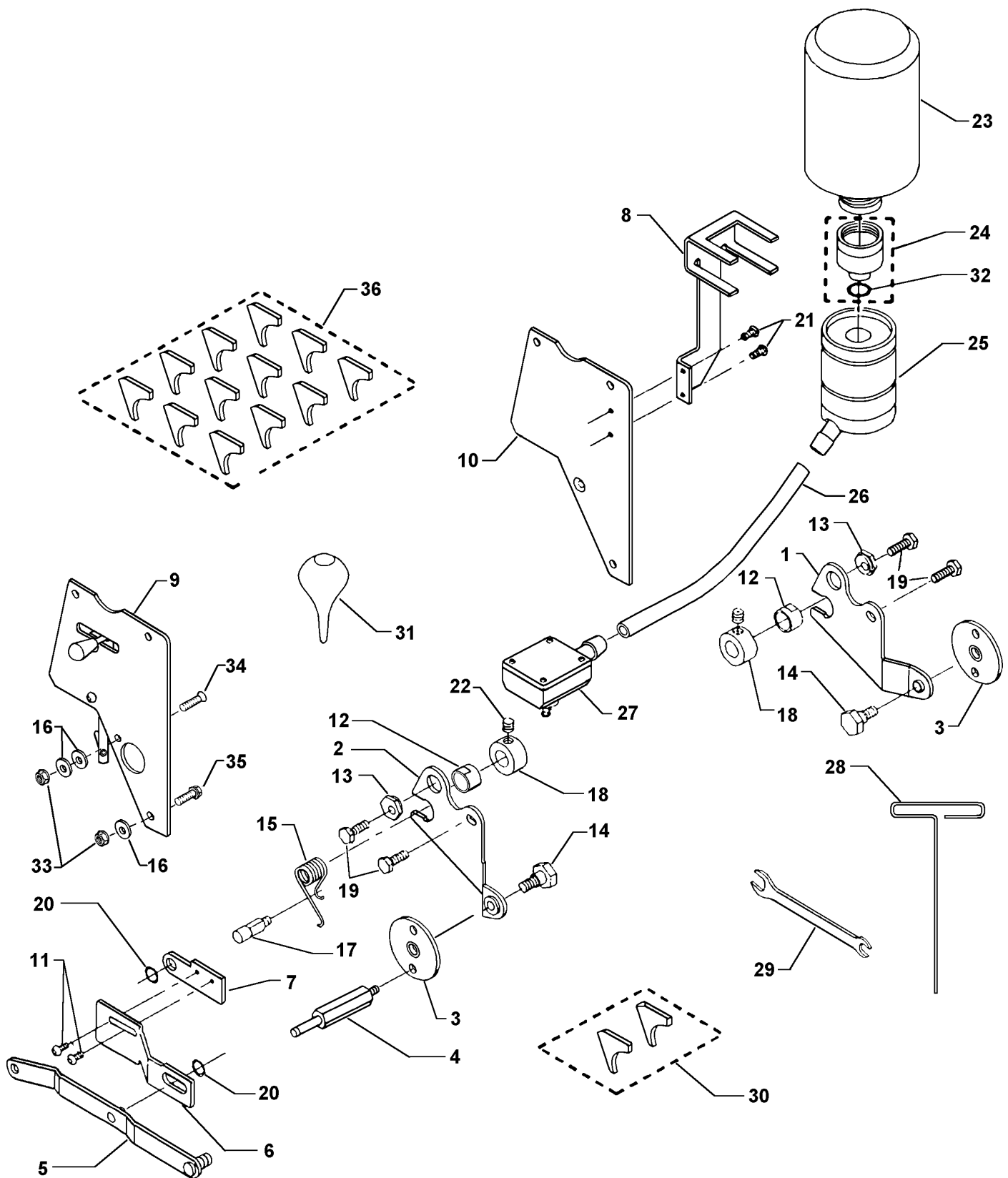
FIGURE 14 Dampener - Part II
