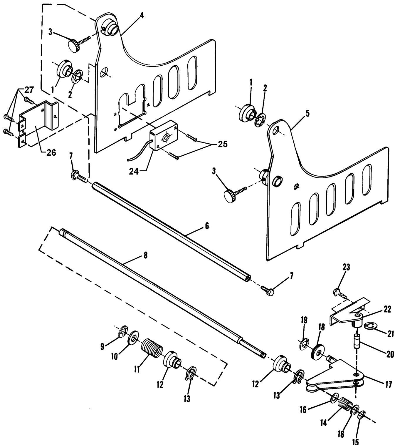
FIGURE 78 Paper Guides Chain Delivery
